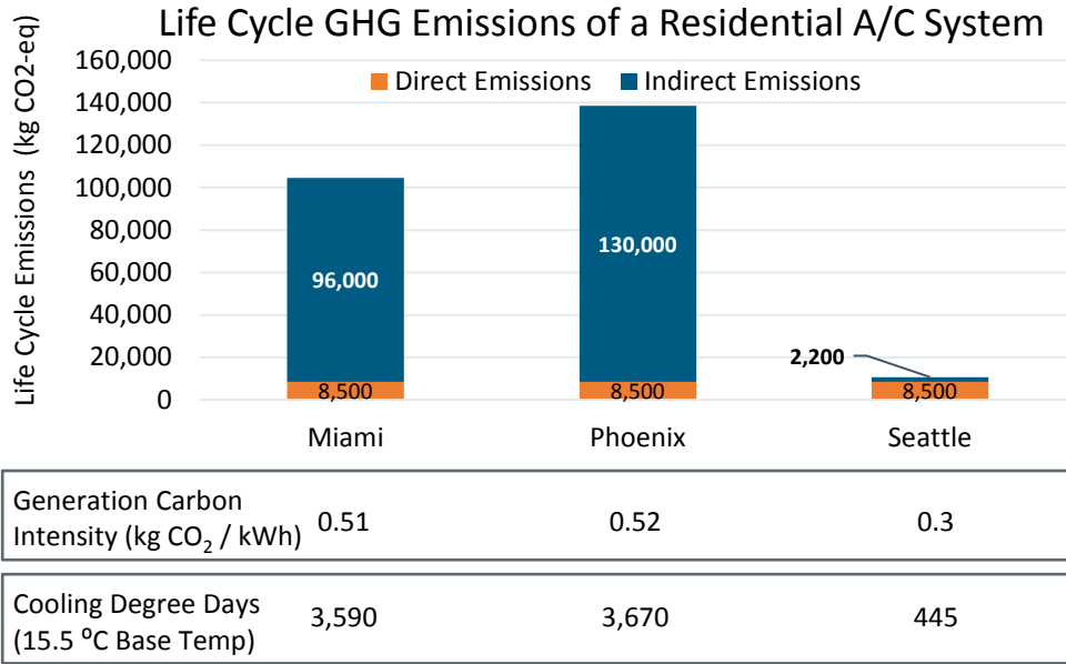
Figure 3-3: Life cycle GHG emissions of residential air-conditioning systems 55
