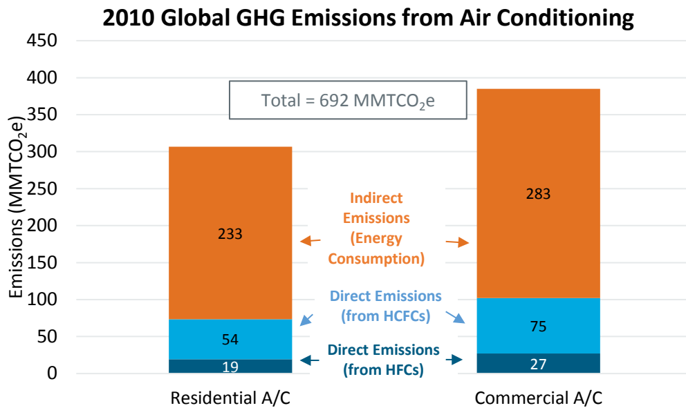
Sources: IPCC (2014), 32 World Bank (2014), 209 EPA (2012), 210 Xiang, et al. (2014), 211 ICF (2007) 212 Figure B-1: Estimated global GHG emissions from air-conditioning systems in 2010
